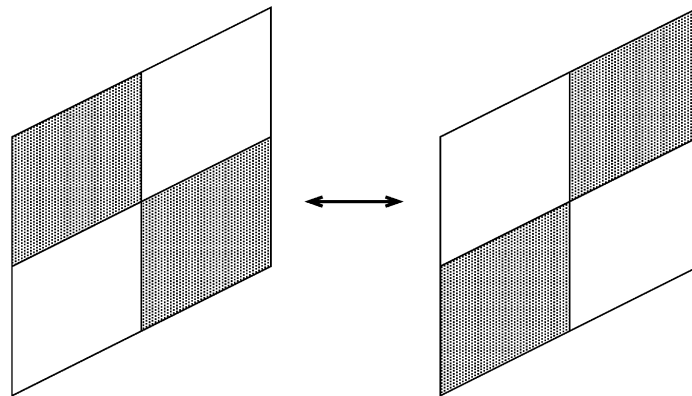
Fig. 1. Two period cells of a generalized checkerboard.
